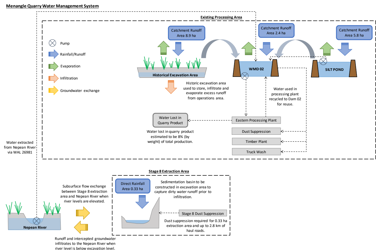
Figure 5.6 Water management system schematic
